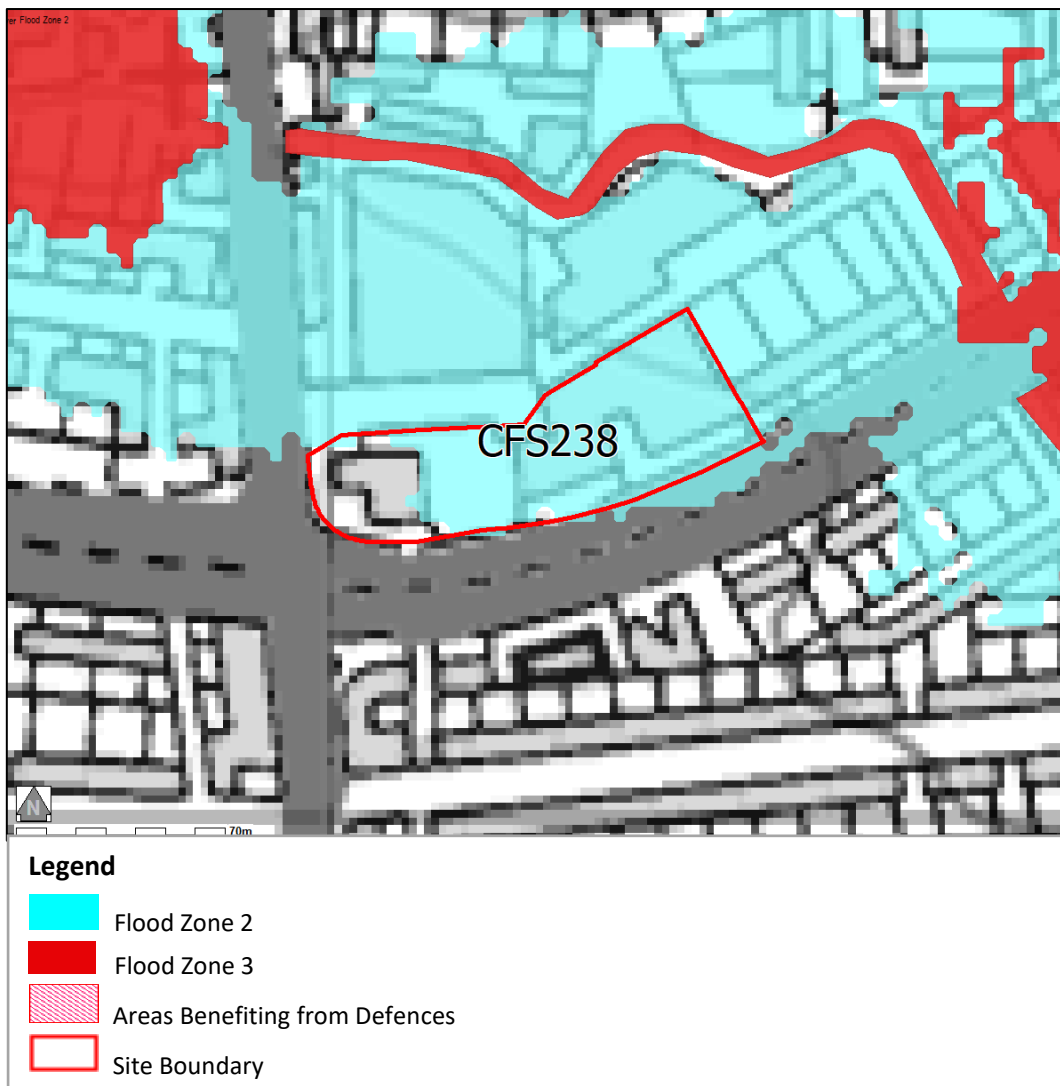
Figure 8 Flood Zones
