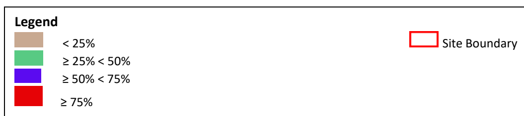
Figure 4 Susceptibility to Groundwater Flooding
