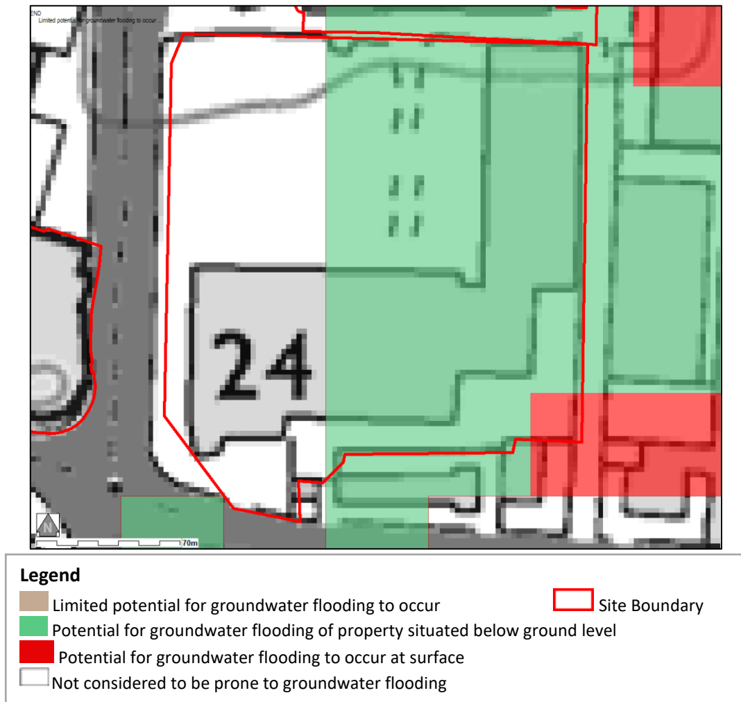
Figure 3 Groundwater Flooding
