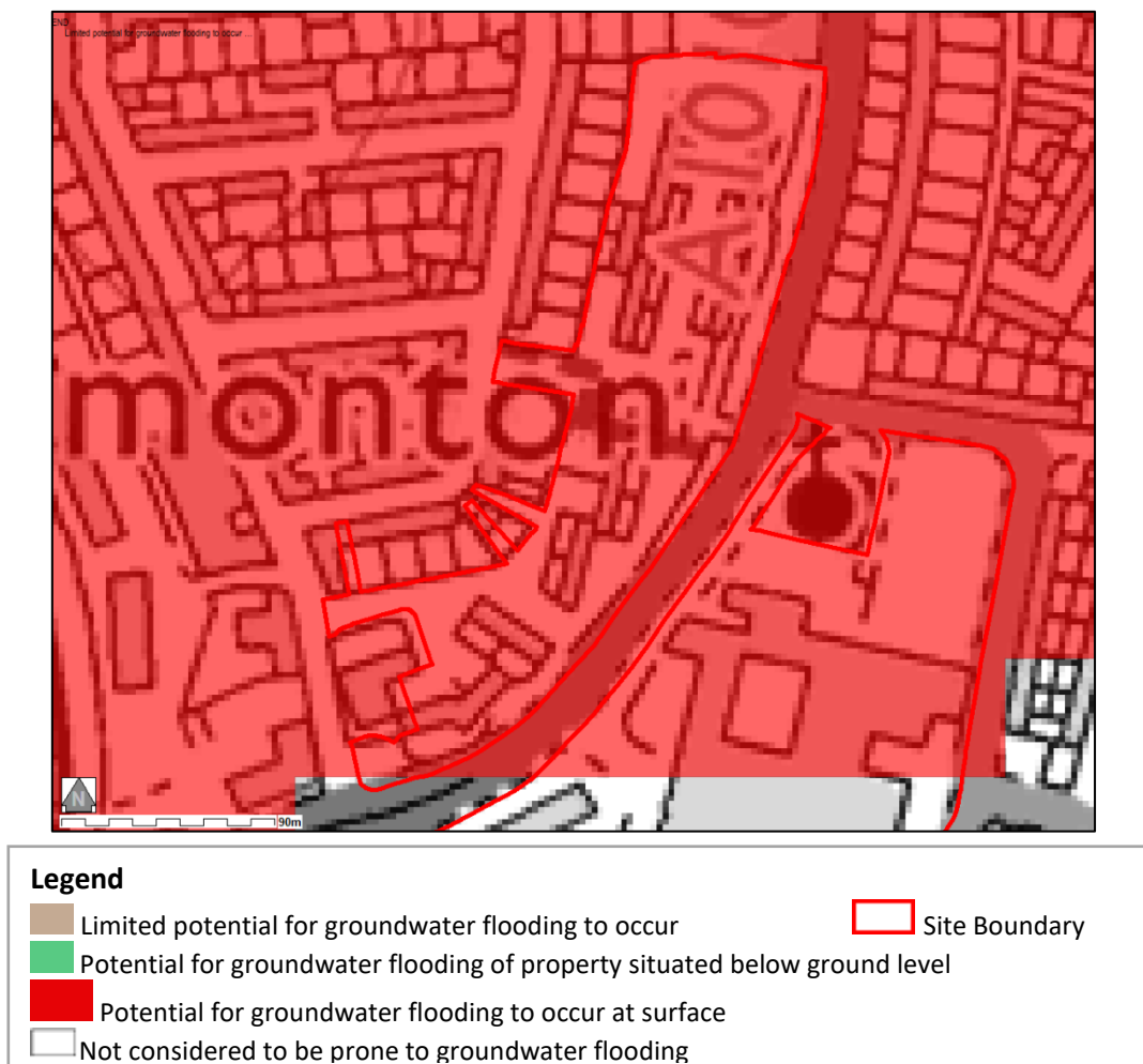
Figure 3 Groundwater Flooding
