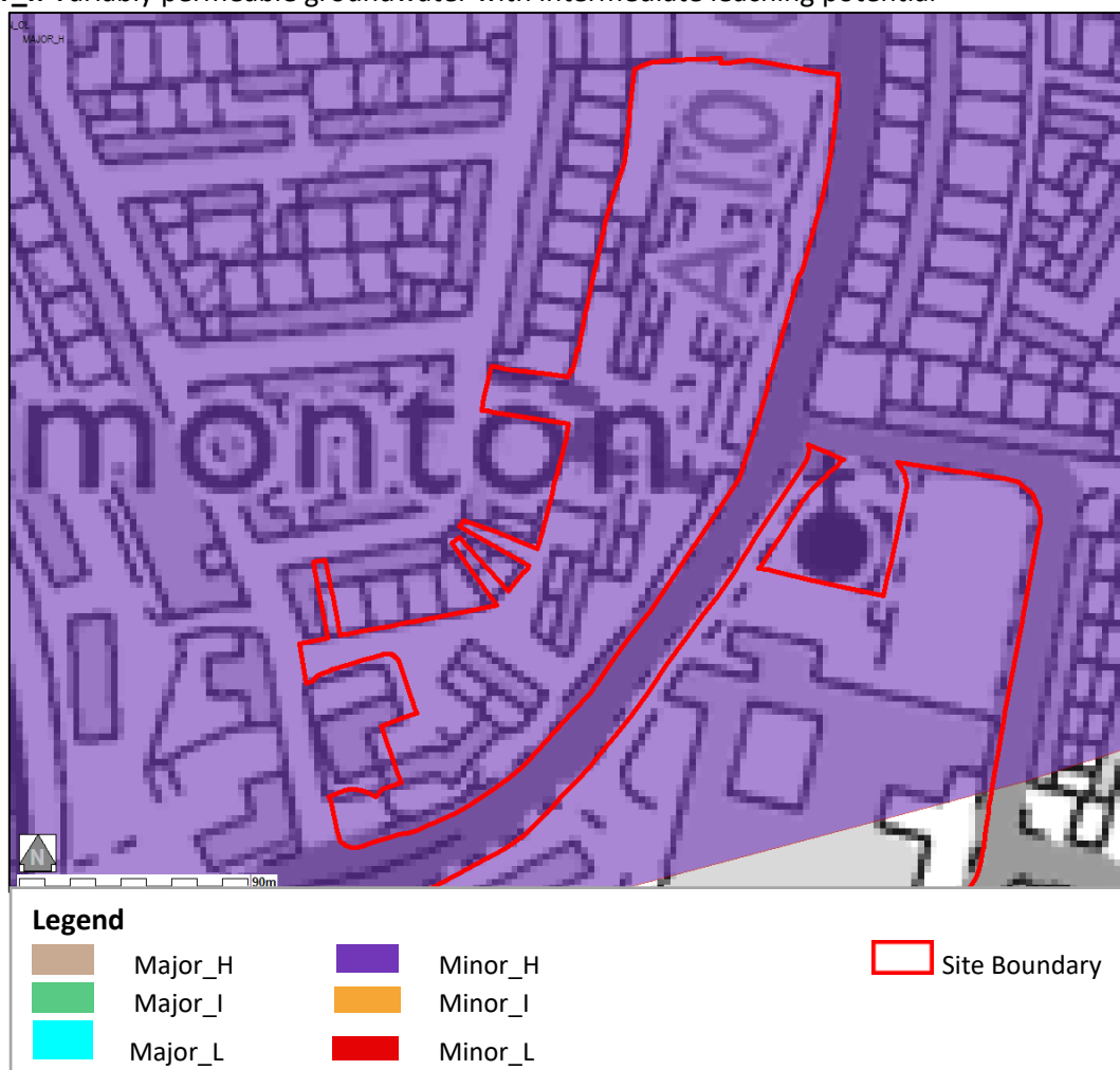
Figure 6 Groundwater Vulnerability
