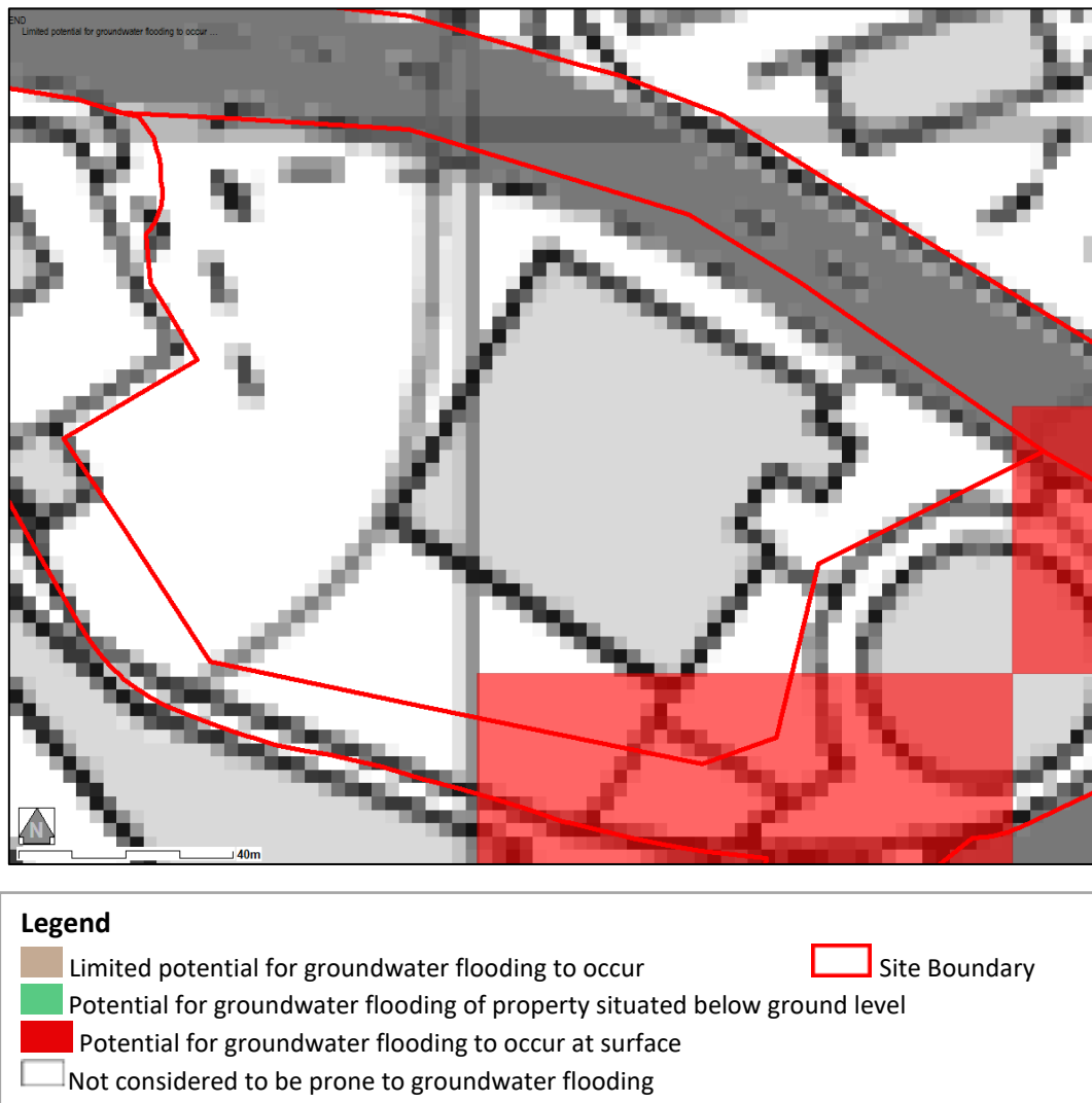
Figure 3 Groundwater Flooding
