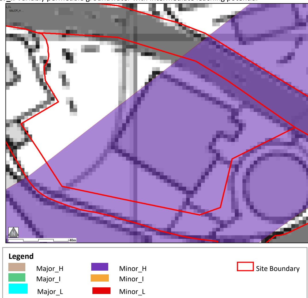
Figure 6 Groundwater Vulnerability
