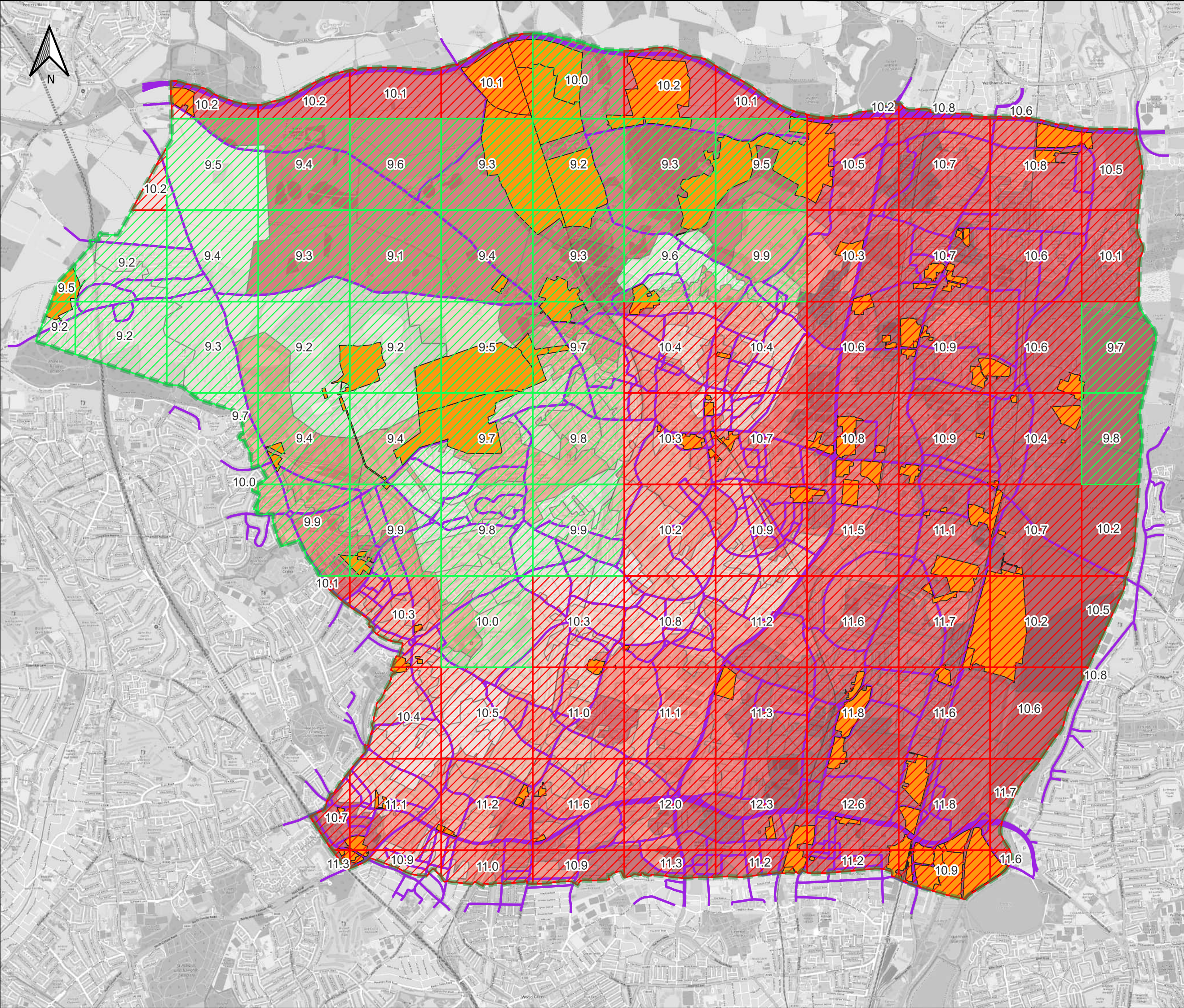
Figure A-2: Predicted 2030 PM 2.5 Background Concentration
