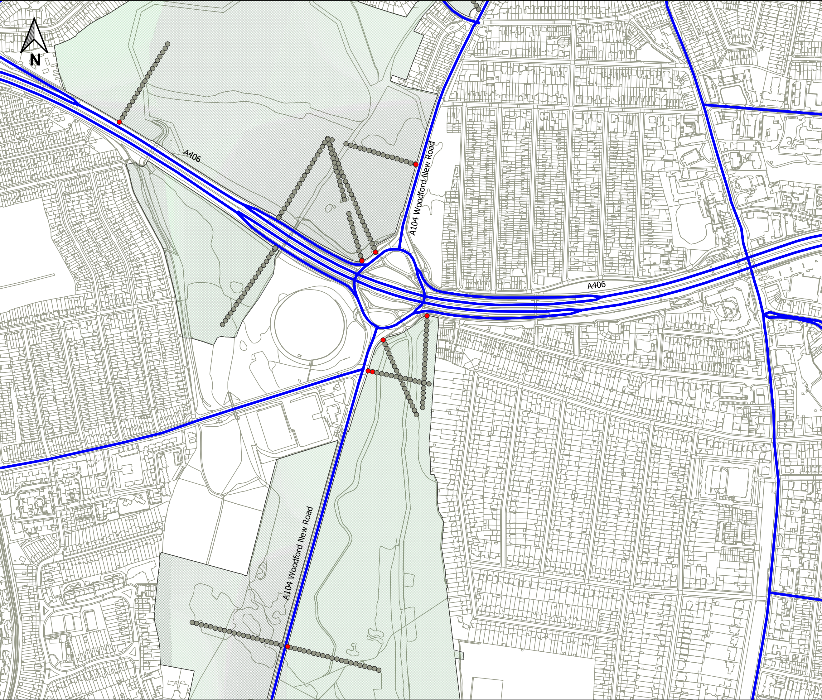
Figure A-6: Epping Forest SAC A406 North Circular and Woodford New Road (NH 3 )
