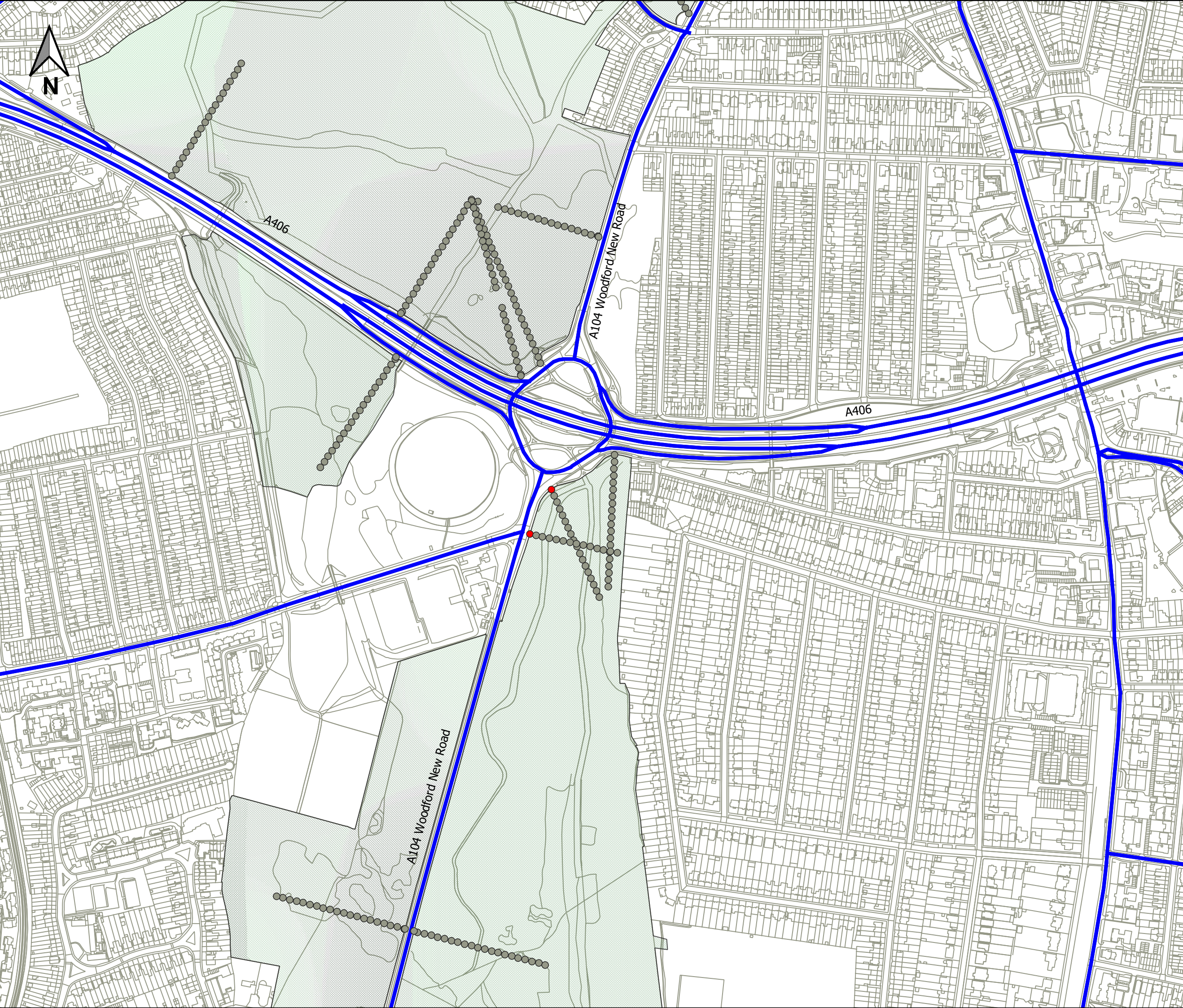
Figure A-5: Epping Forest SAC A406 North Circular and Woodford New Road (NOx)
