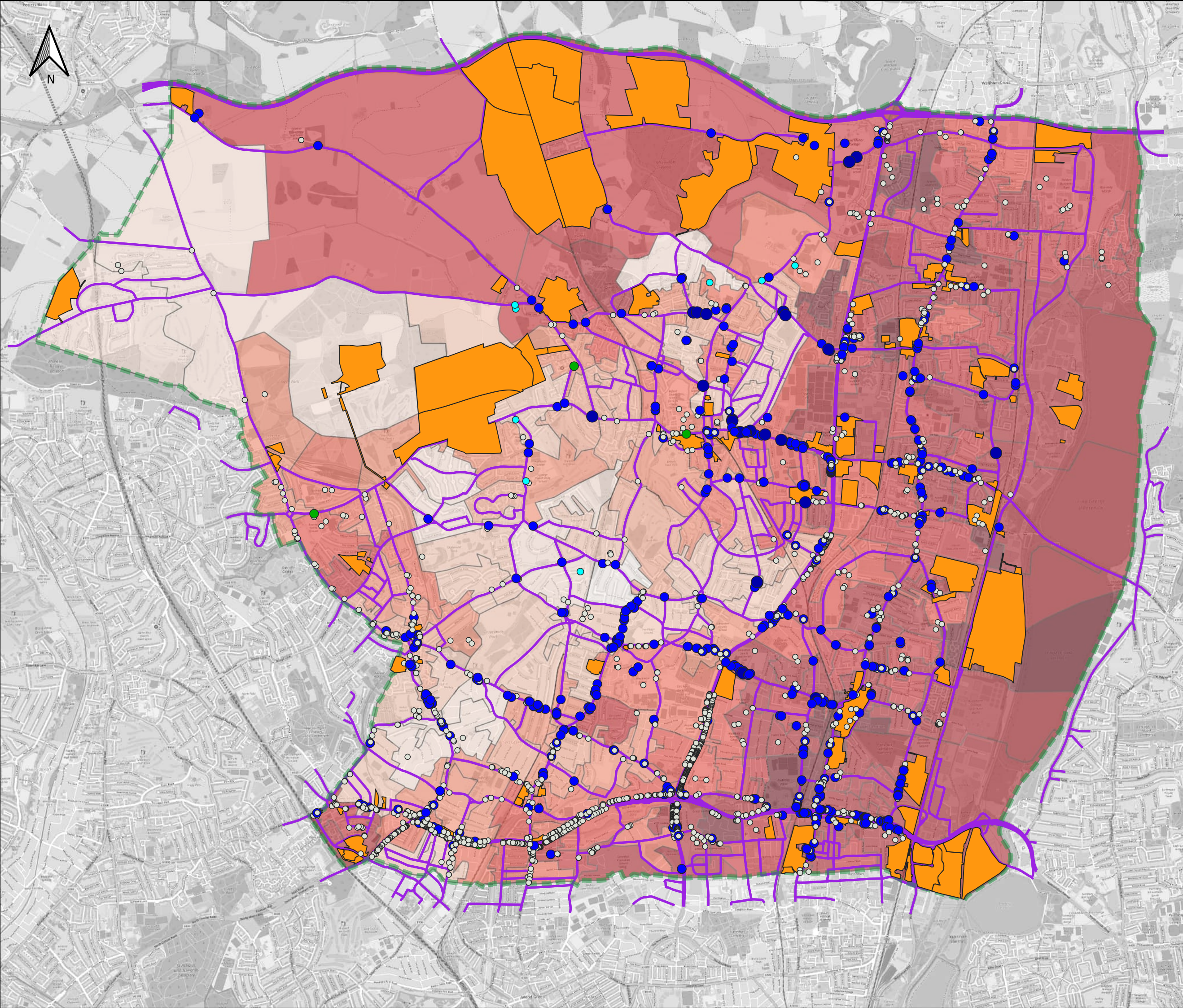
Figure A-4: Impact on Annual Mean PM 2.5 Concentrations Relative to Mayor of London's Target for 2030
