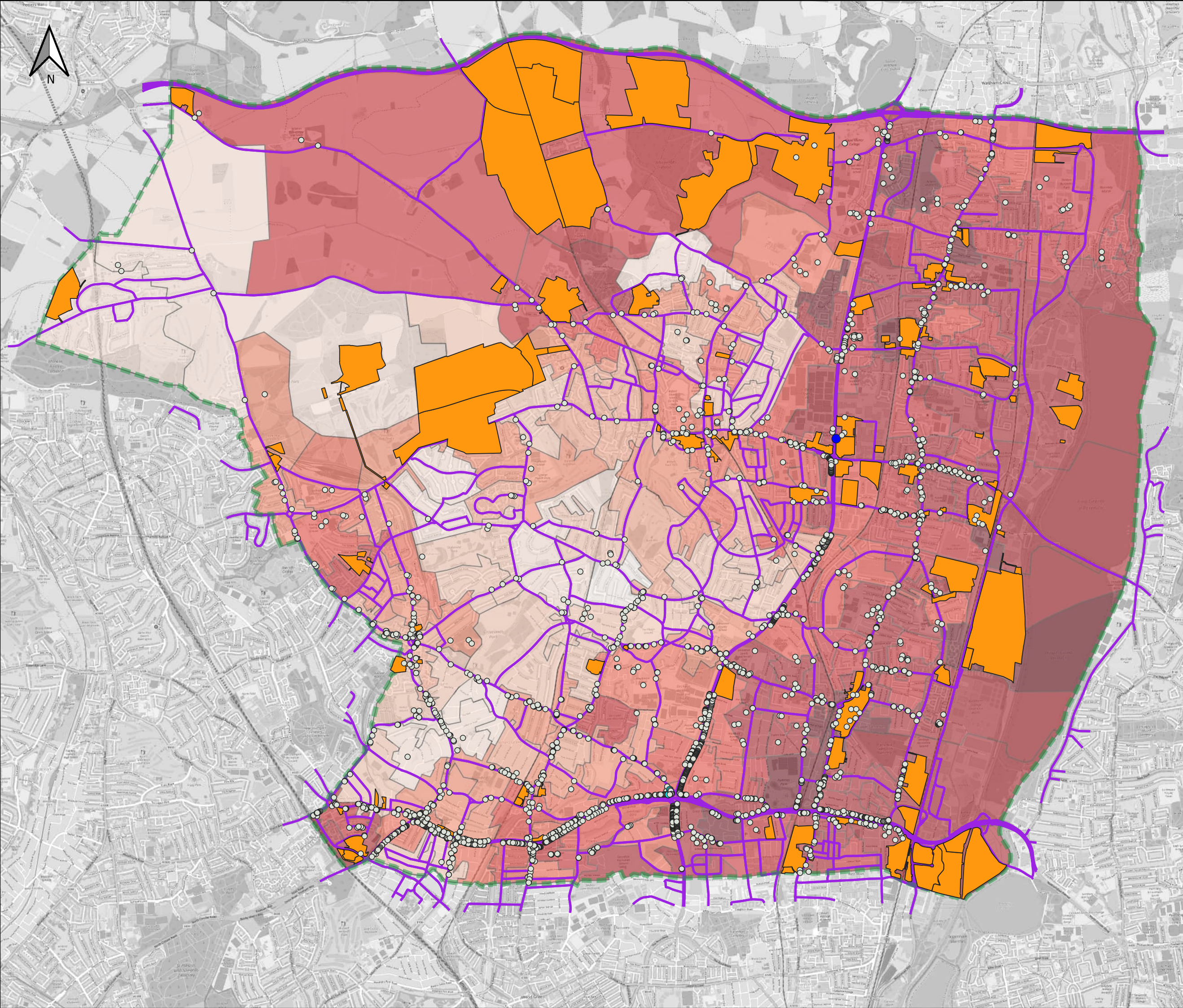
Figure A-3: Impact on Annual Mean NO 2 Concentrations
