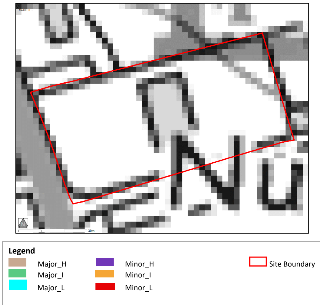
Figure 6 Groundwater Vulnerability
