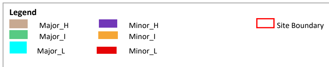
Figure 6 Groundwater Vulnerability
