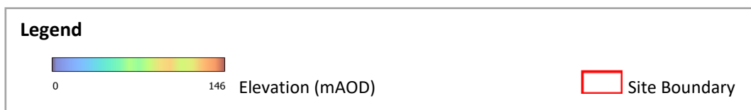
Figure 1 Topography
