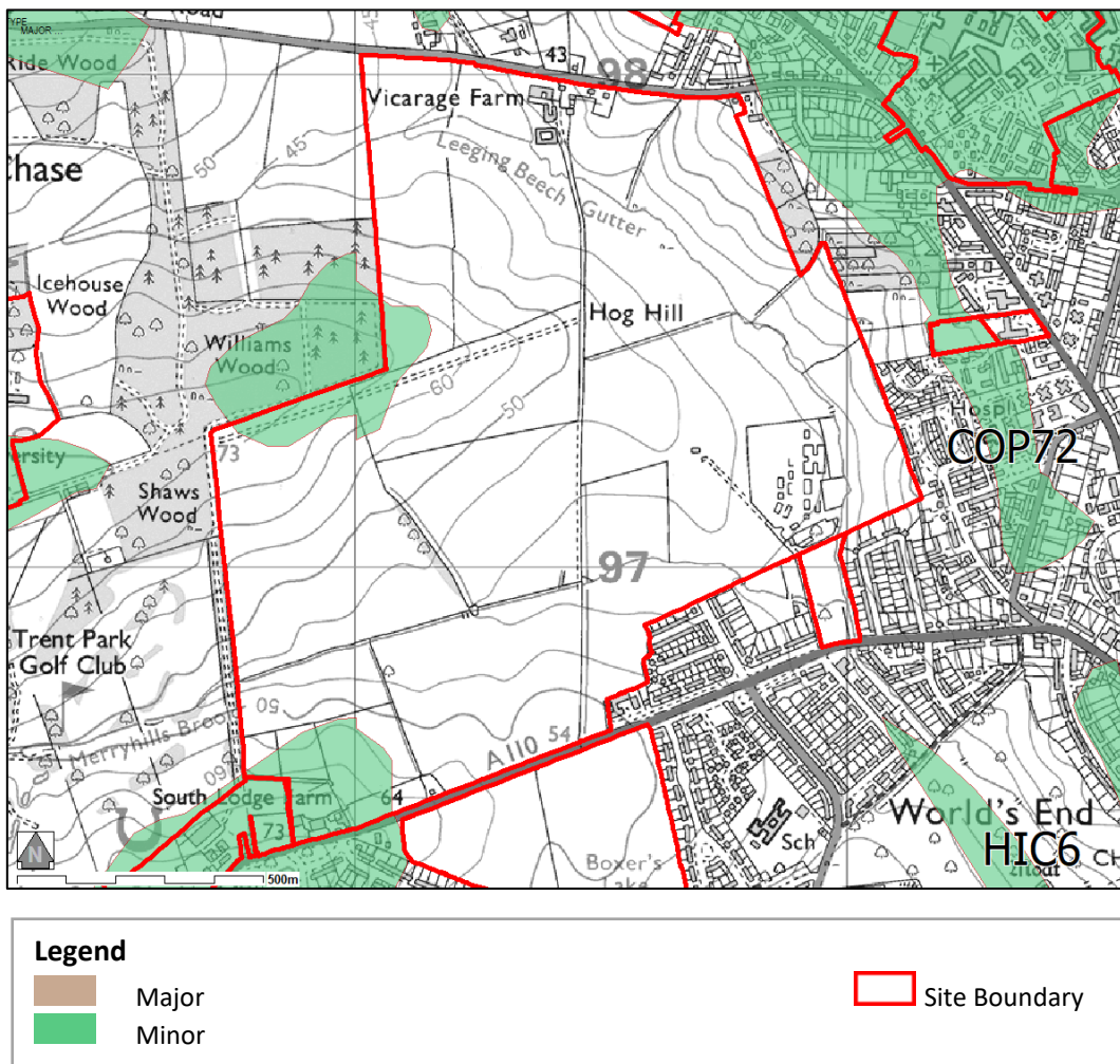
Figure 5 Groundwater Resources
