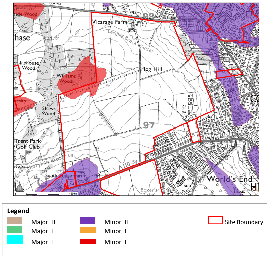
Figure 6 Groundwater Vulnerability
