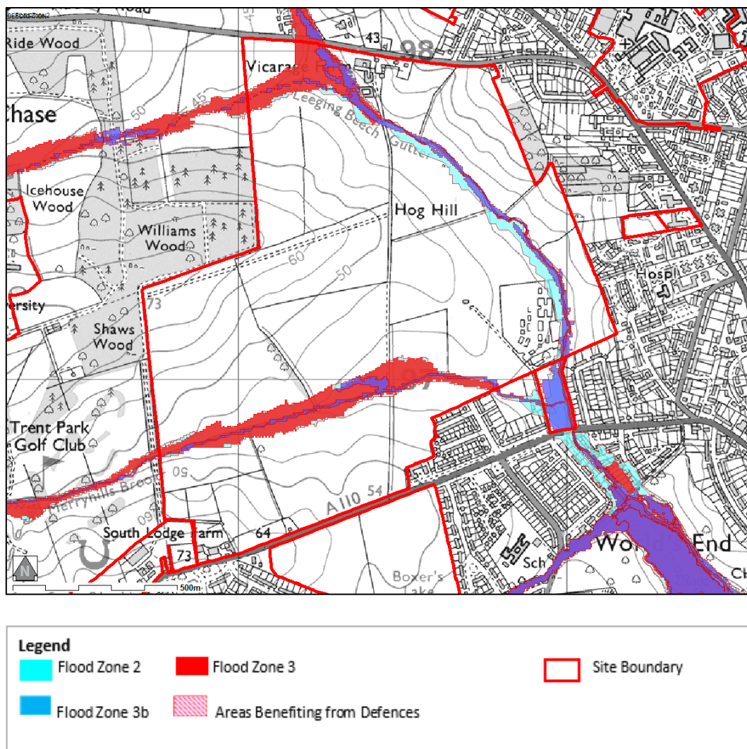
Figure 9 Flood Zones
