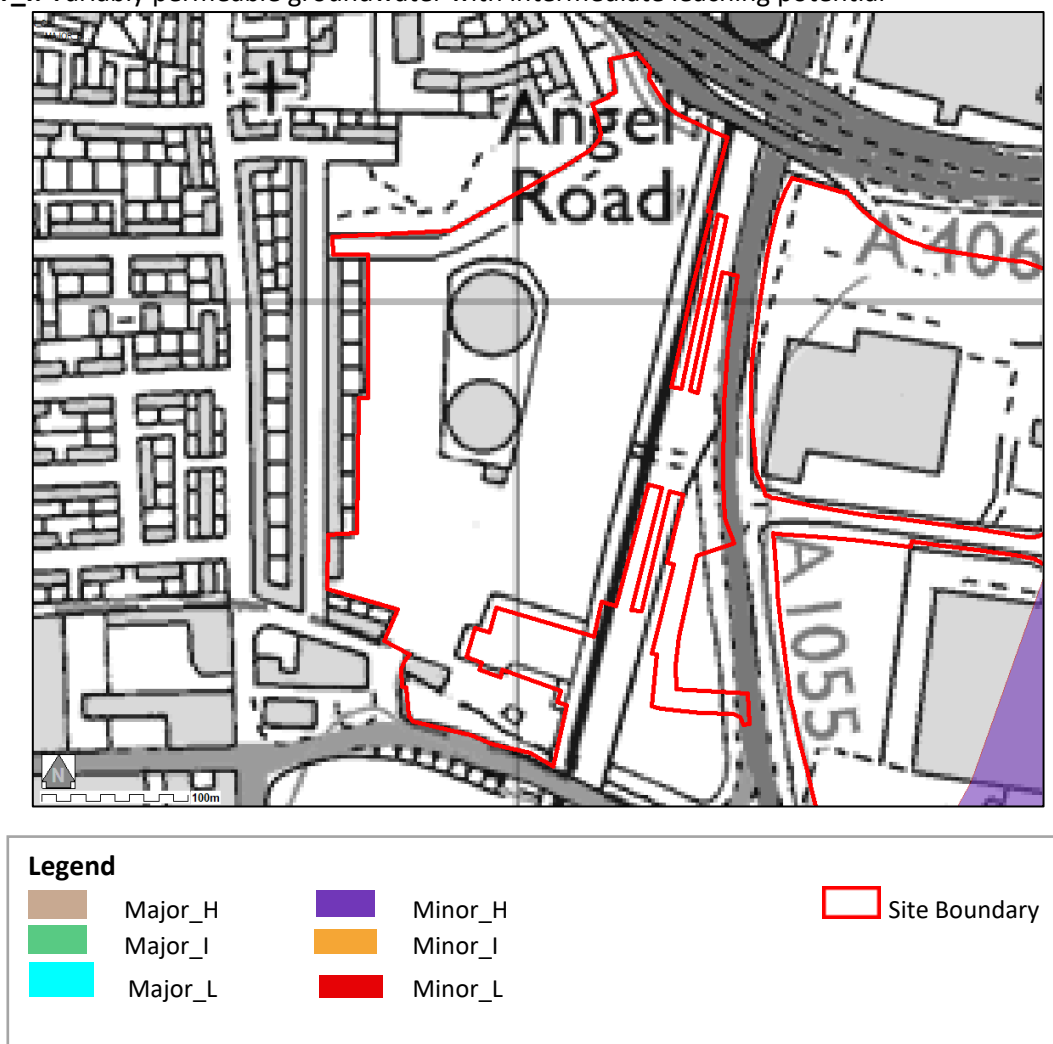
Figure 6 Groundwater Vulnerability
