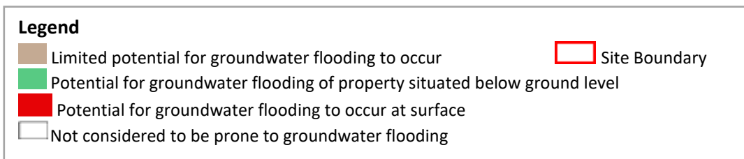
Figure 3 Groundwater Flooding
