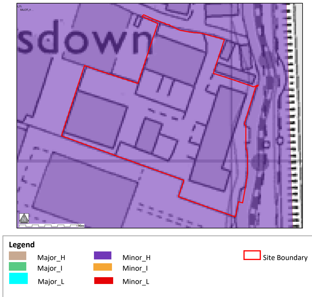
Figure 6 Groundwater Vulnerability
