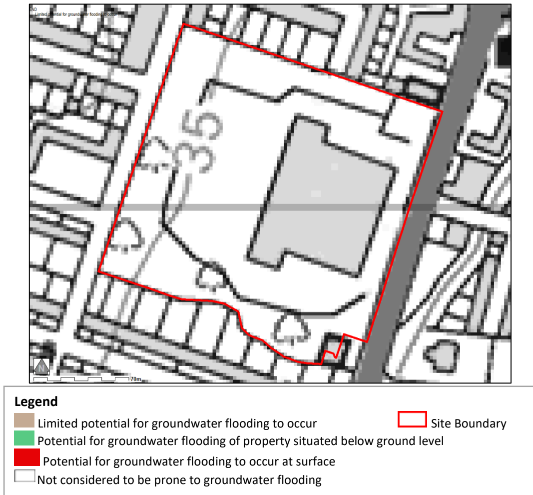
Figure 3 Groundwater Flooding
