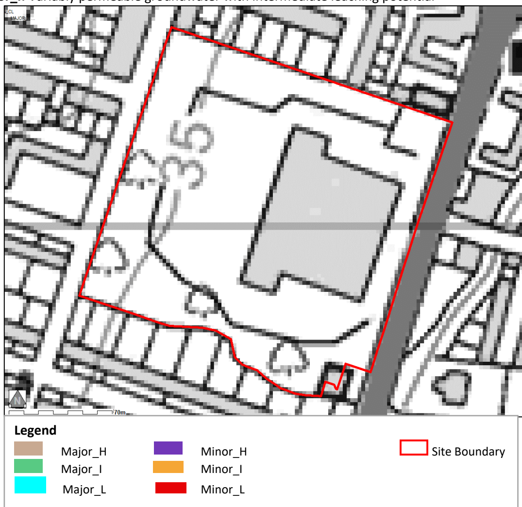
Figure 6 Groundwater Vulnerability
