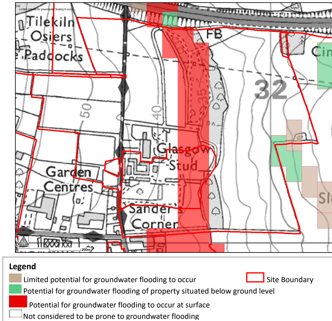
Figure 3 Groundwater Flooding
