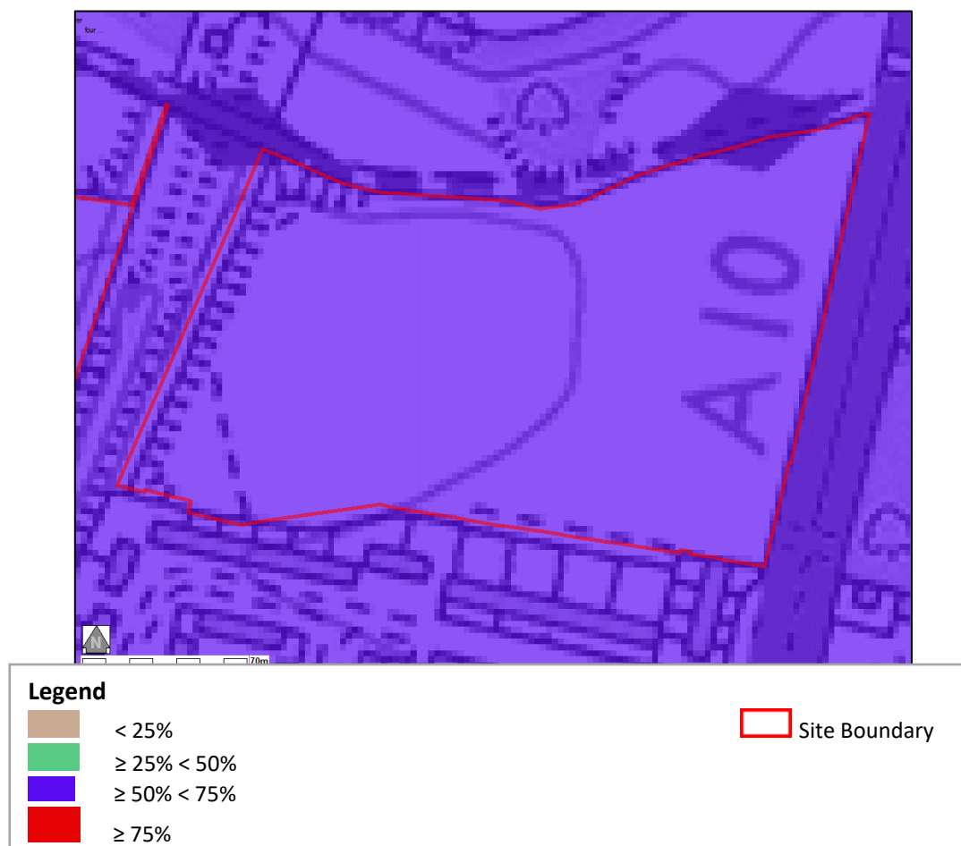
Figure 4 Susceptibility to Groundwater Flooding
