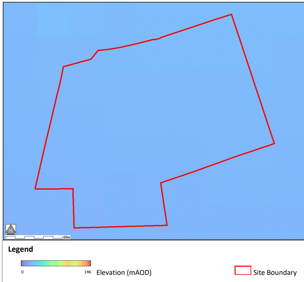
Figure 1 Topography
