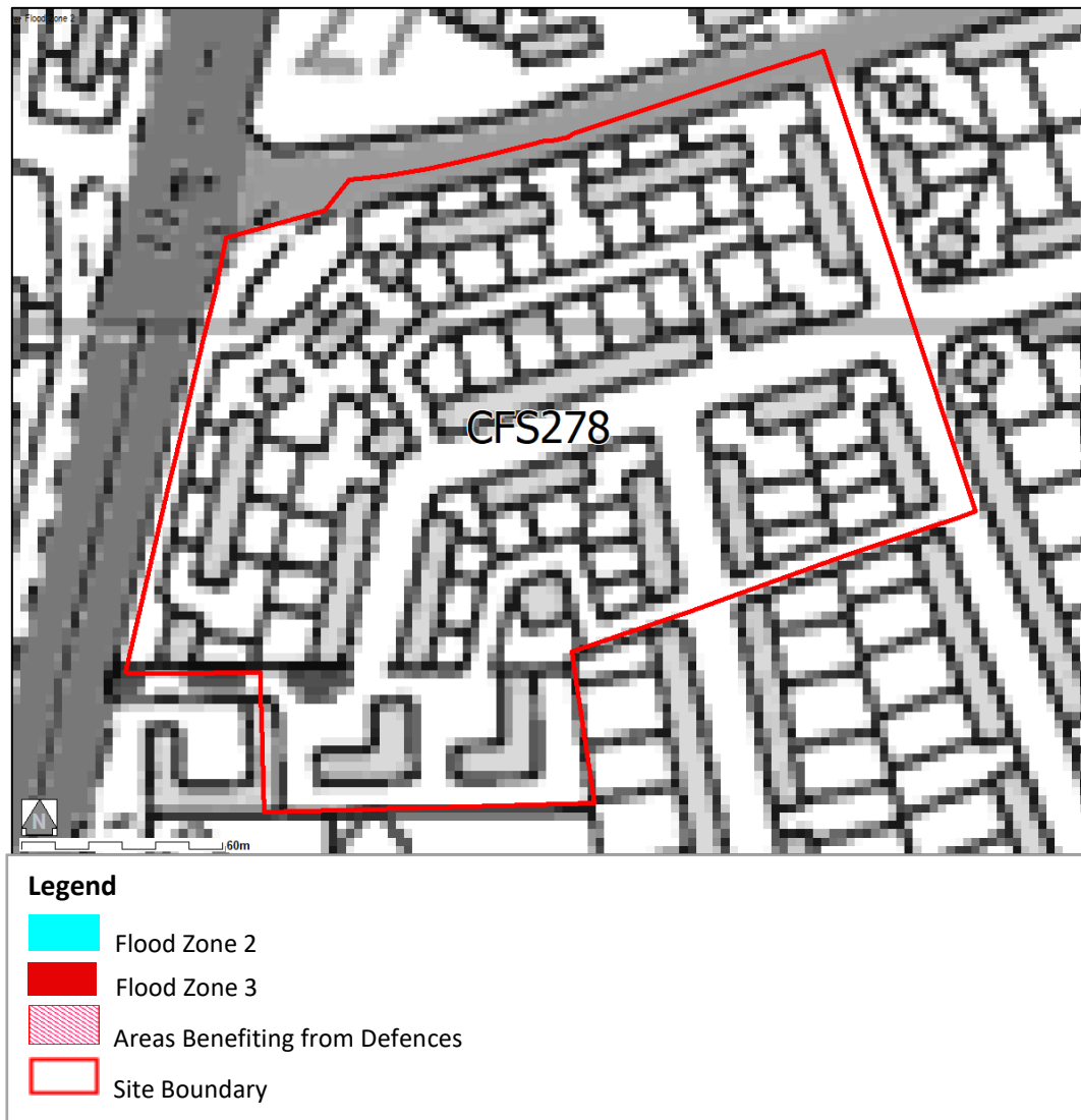
Figure 8 Flood Zones
