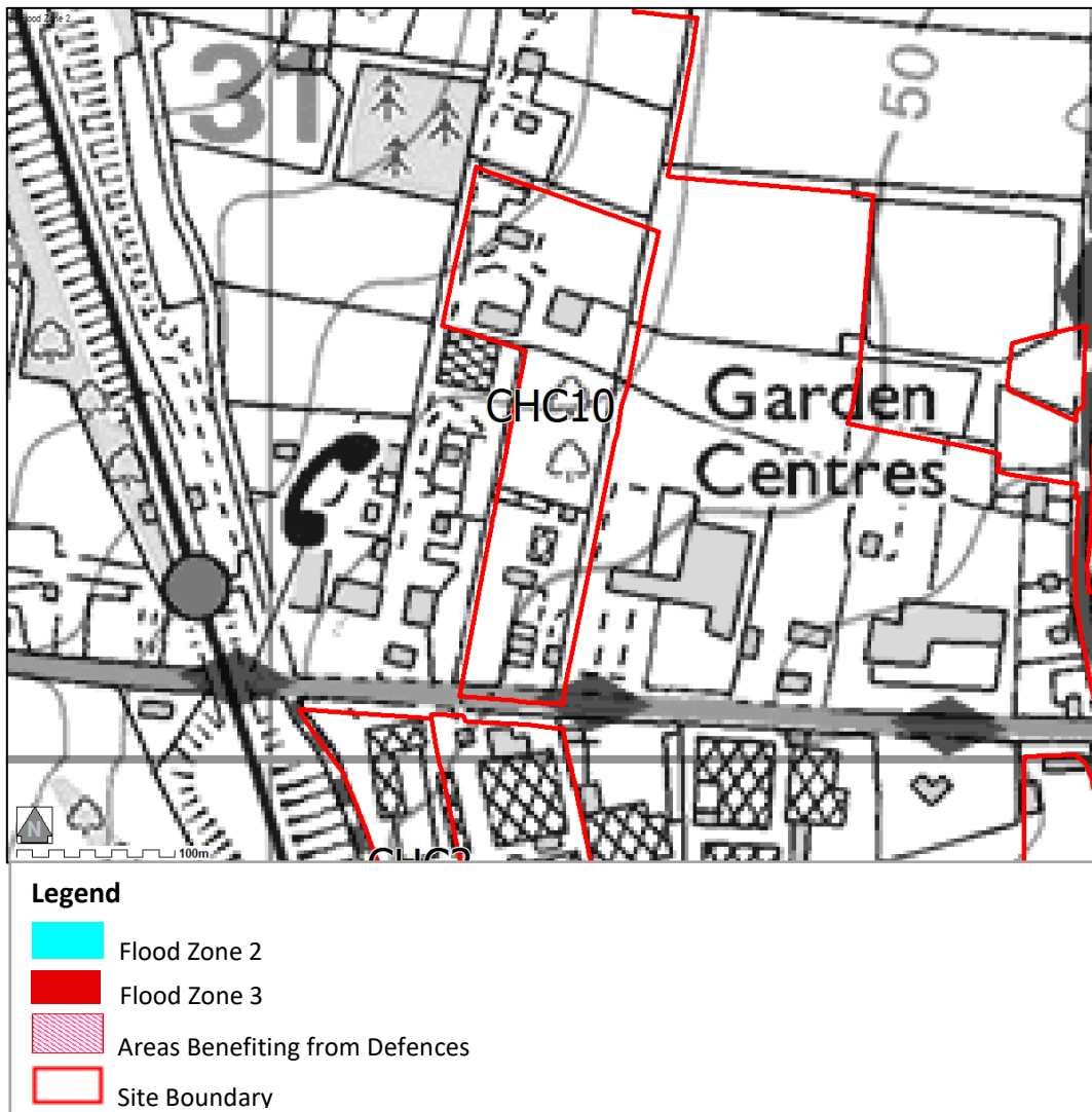
Figure 8 Flood Zones
