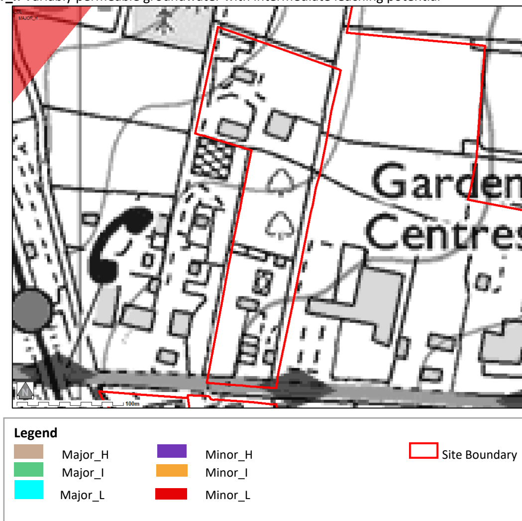
Figure 6 Groundwater Vulnerability
