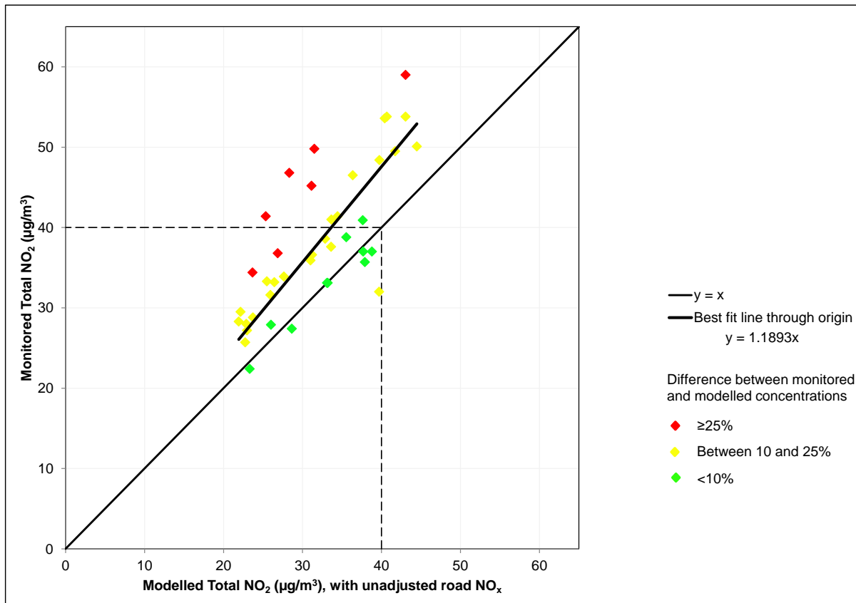
Figure B-1: Comparison between Monitored Total NO 2 and Modelled Total NO 2 (before adjustment)
