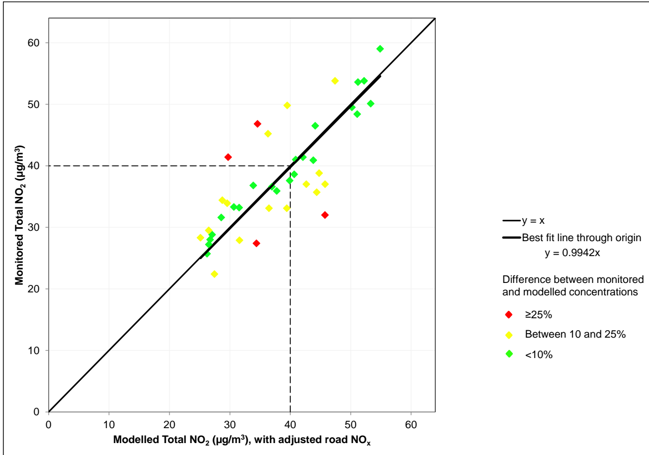
Figure B-3: Comparison of measured total NO 2 with modelled total NO 2 (with adjusted road-NO x )
