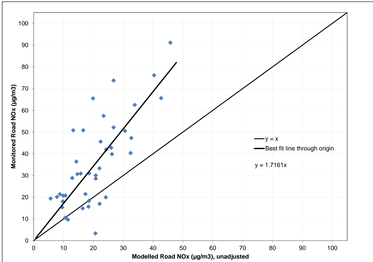
Figure B-2: Comparison of measured road-NO x with unadjusted modelled road-NO x
