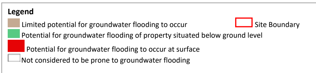
Figure 3 Groundwater Flooding
