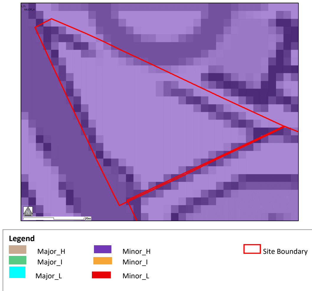
Figure 6 Groundwater Vulnerability
