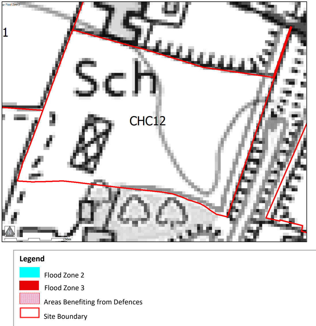
Figure 8 Flood Zones
