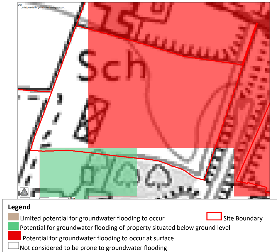
Figure 3 Groundwater Flooding
