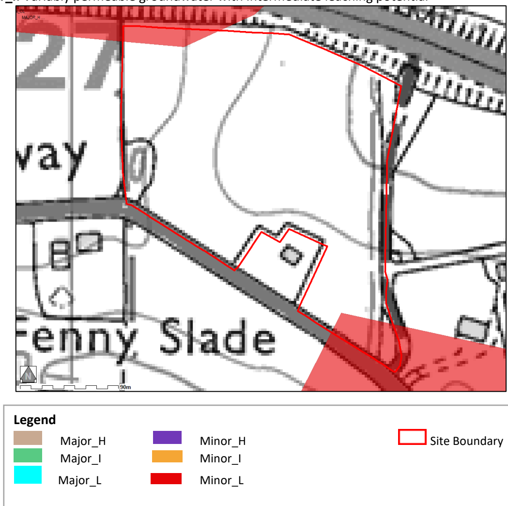
Figure 6 Groundwater Vulnerability
