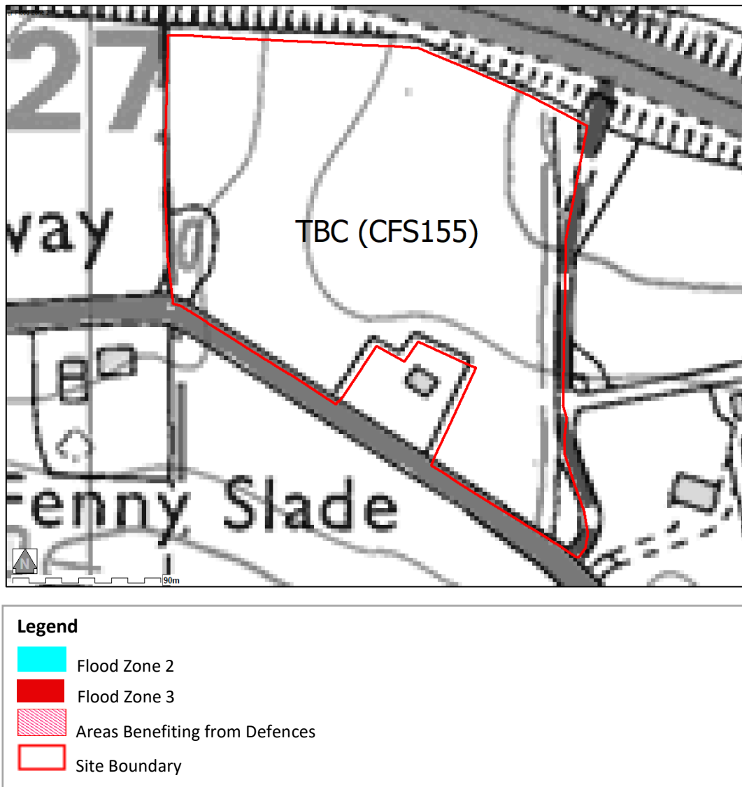
Figure 8 Flood Zones
