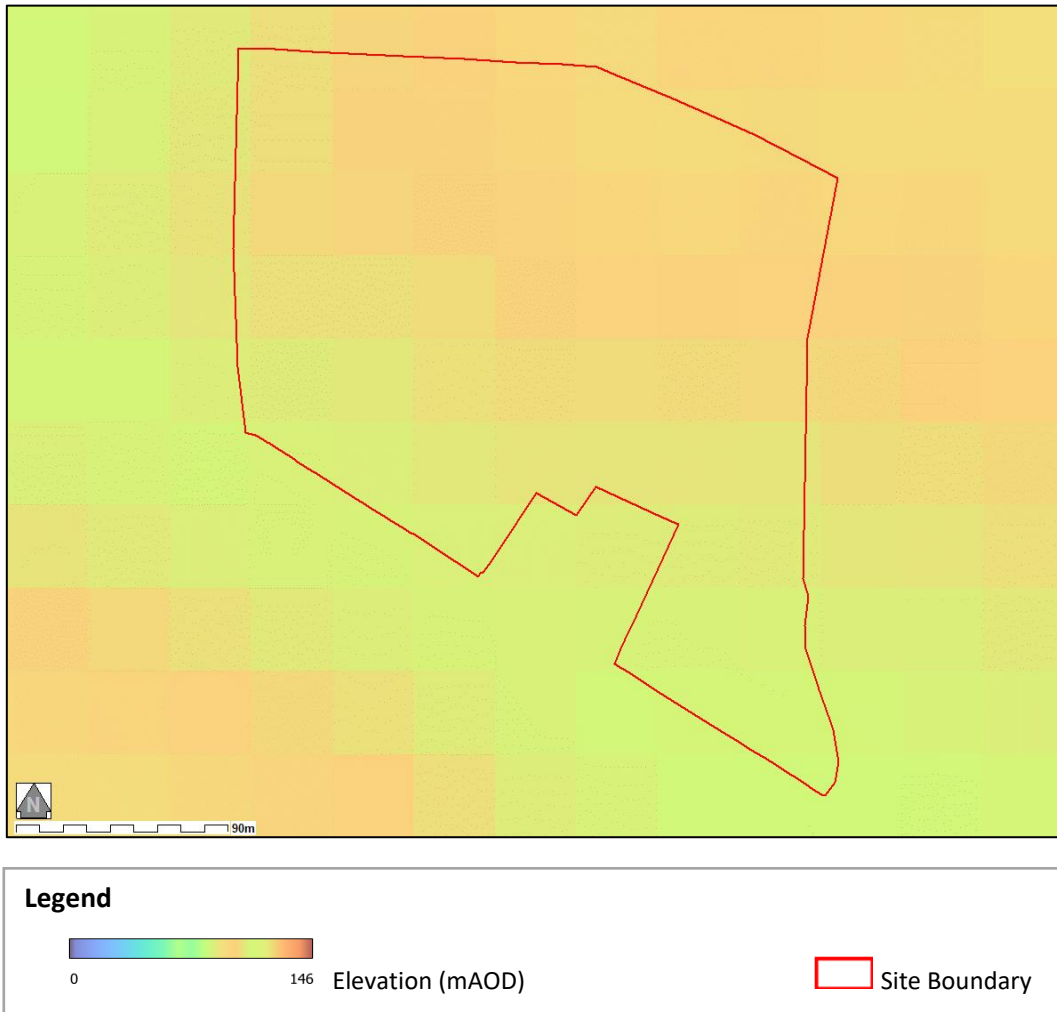
Figure 1 Topography
