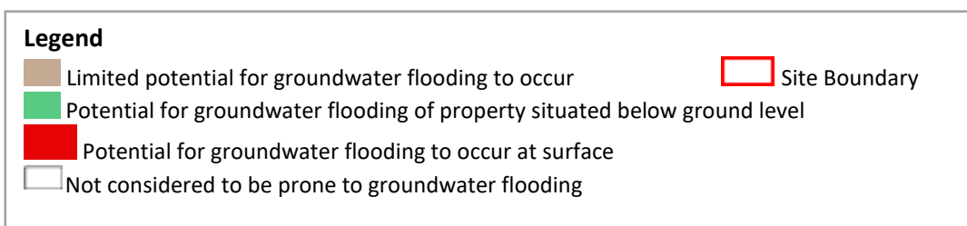
Figure 3 Groundwater Flooding
