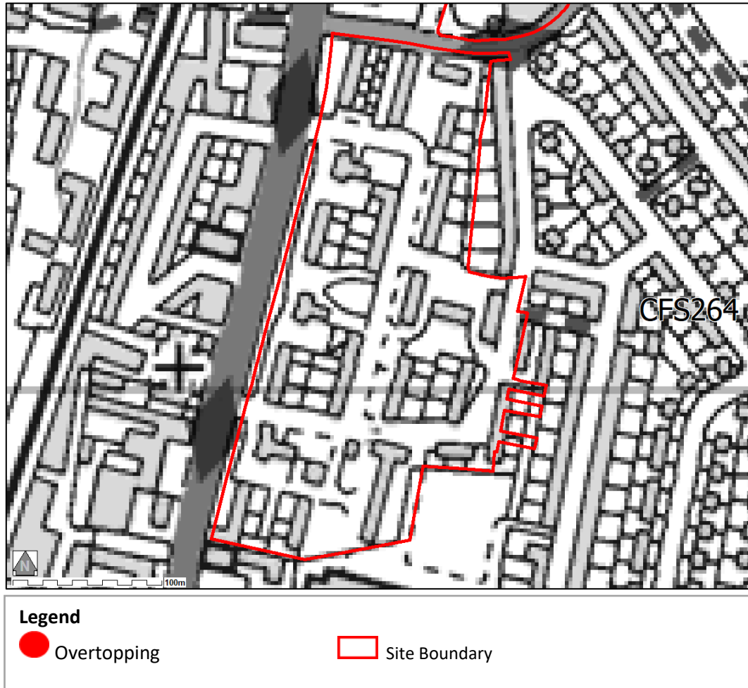
Figure 15 Overtopping
