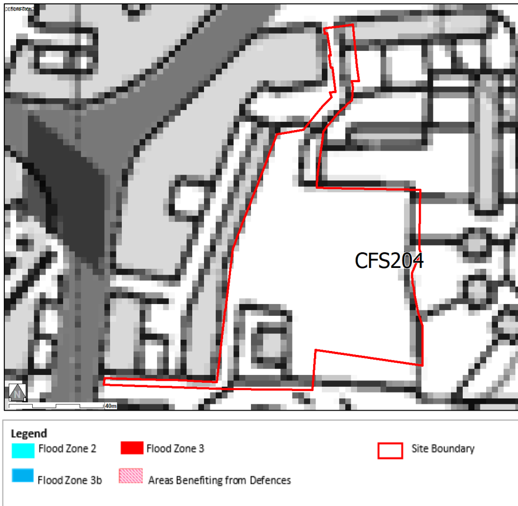
Figure 9 Flood Zones
