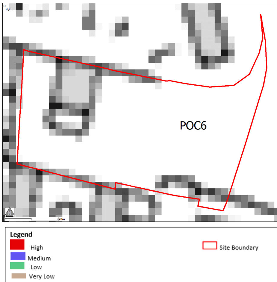
Figure 7 Flood Risk from Rivers and Sea
