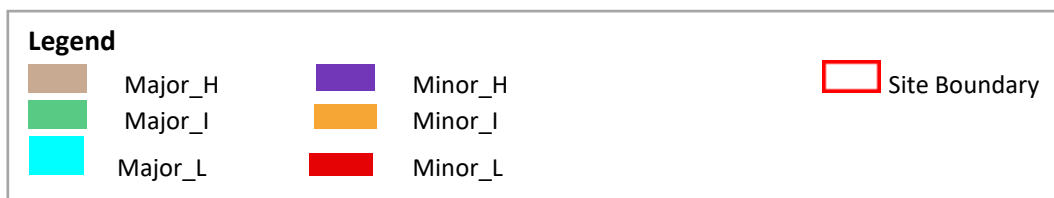
Figure 6 Groundwater Vulnerability
