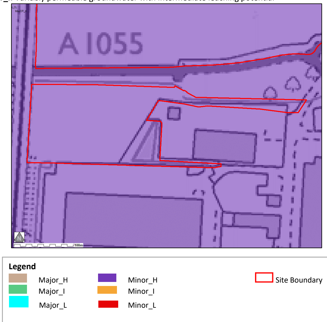
Figure 6 Groundwater Vulnerability
