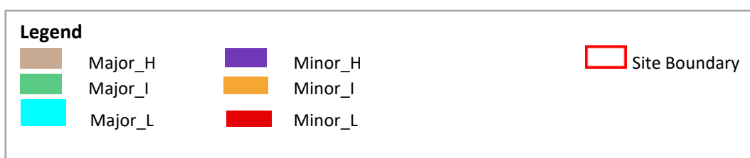
Figure 6 Groundwater Vulnerability
