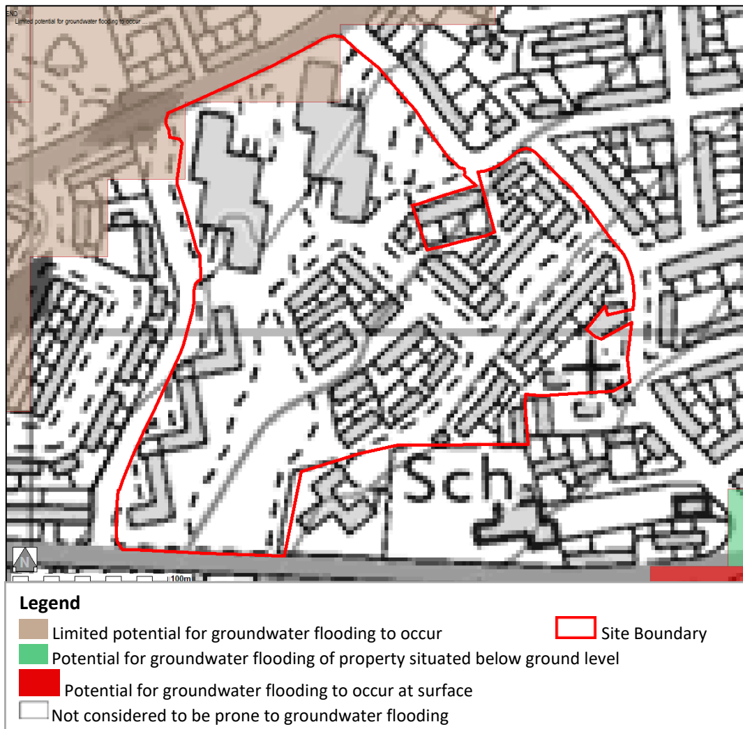
Figure 3 Groundwater Flooding
