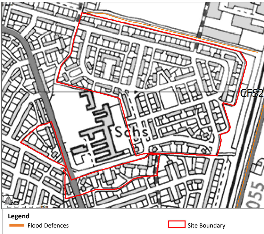
Figure 16 Flood Defences
