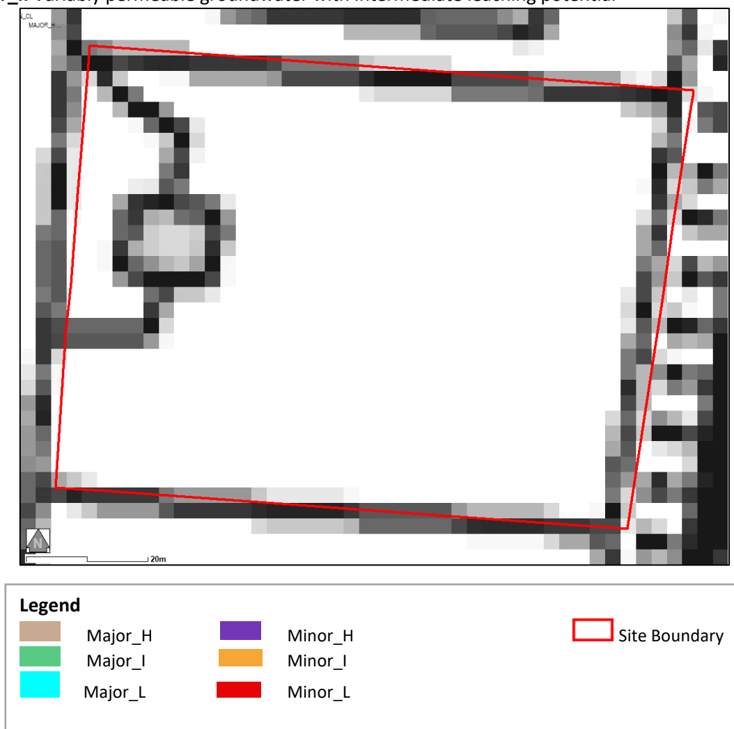
Figure 6 Groundwater Vulnerability
