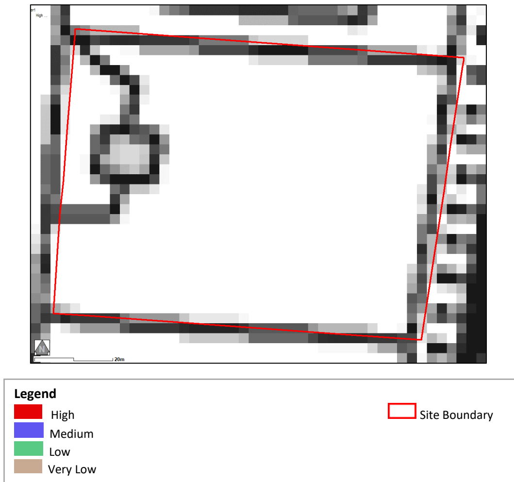
Figure 7 Flood Risk from Rivers and Sea
