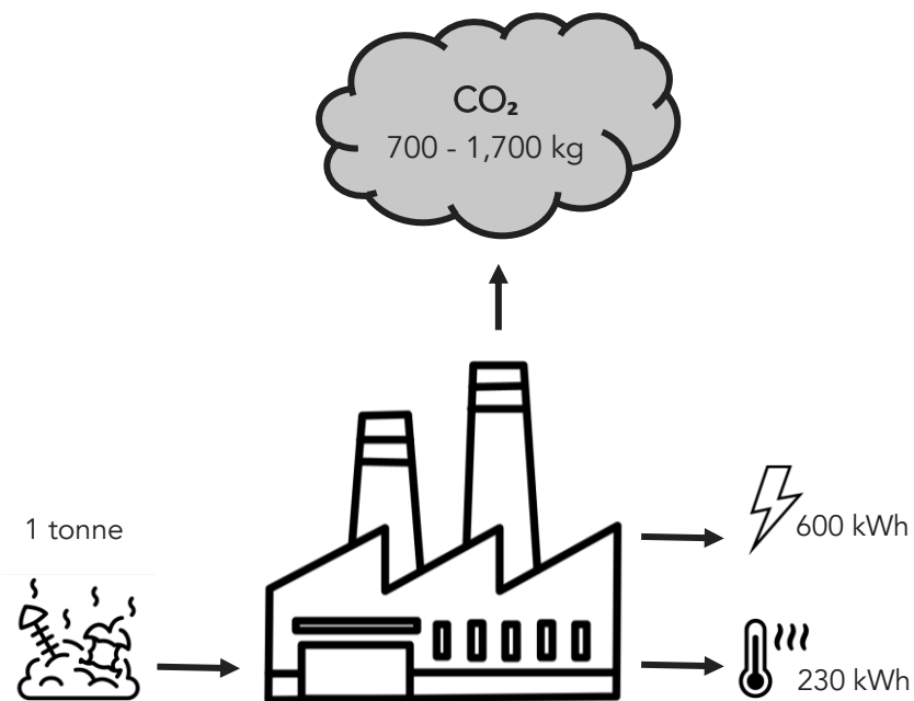
Diagram showing electricity, heat, and carbon dioxide produced through the combustion of 1 tonne of municipal solid waste in a typical waste to energy plant.
