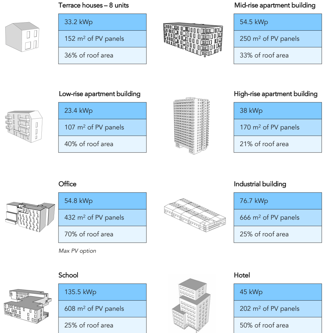
Figure 4.3 – Summary of PV assumptions confirming total PV panel area and kWp output
